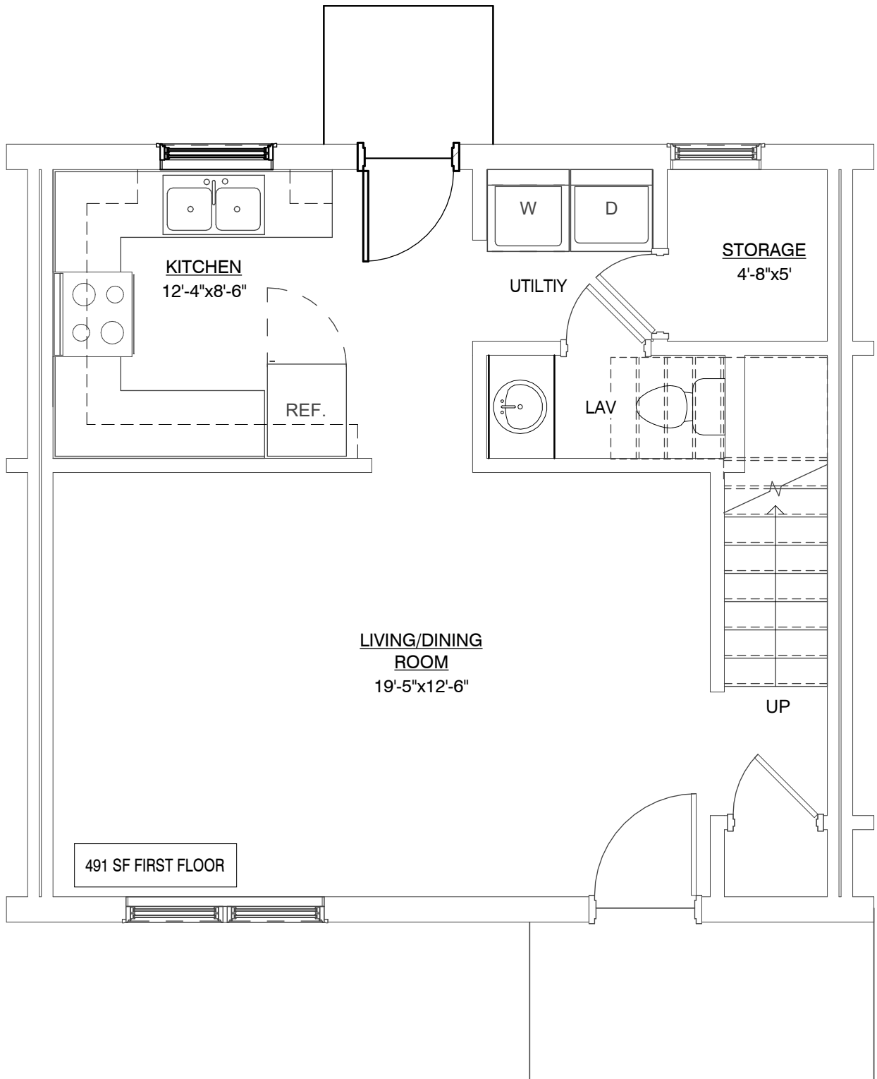
TN090-003 - 3BR - FIRST FLOOR
