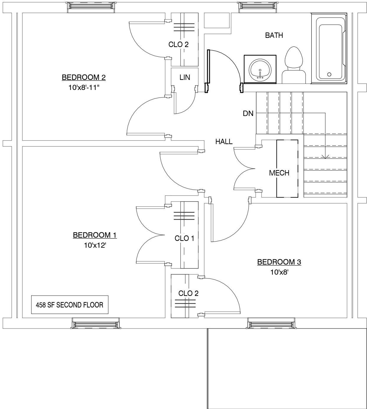
TN090-003 - 3BR - SECOND FLOOR
